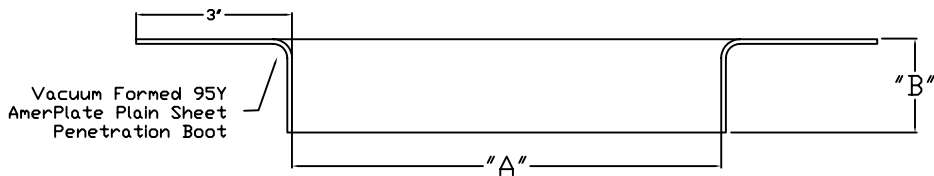
AMERON T-LOCK PIPE PENETRATION BOOT
