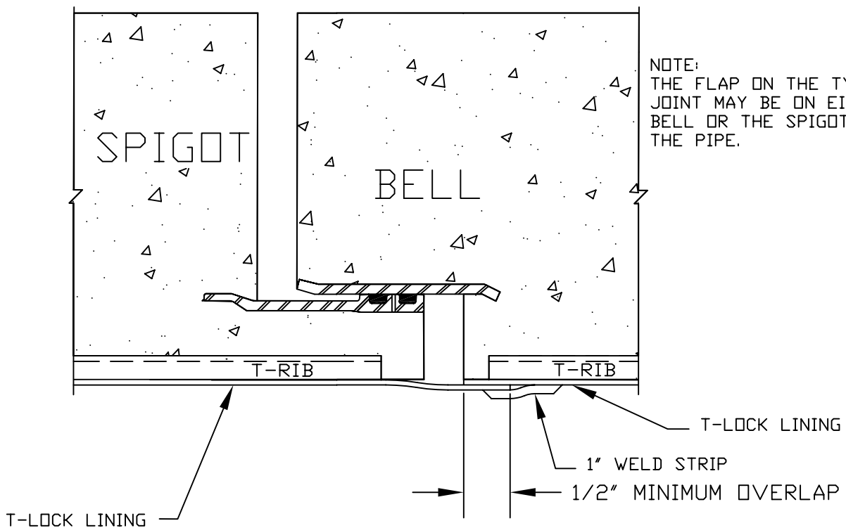
TYPE P-2 JOINT
