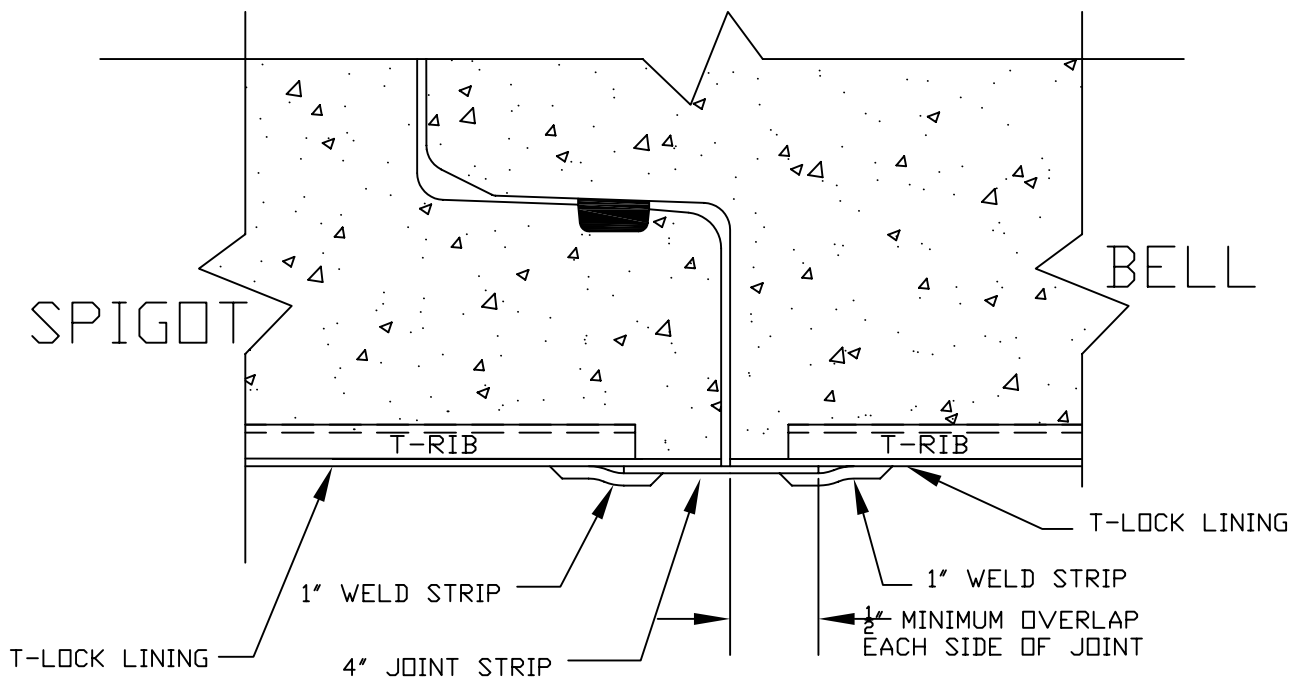
TYPE P-1 JOINT
