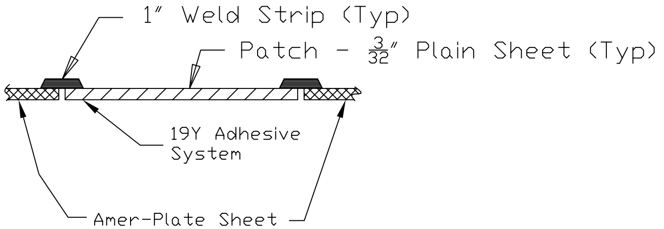
Section B-B
